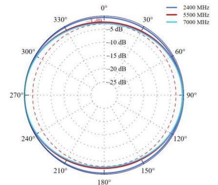
Wi-Fi Azimuth
