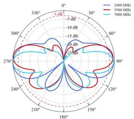
Wi-Fi Elevation
